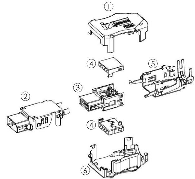
EXPLODED VIEW
